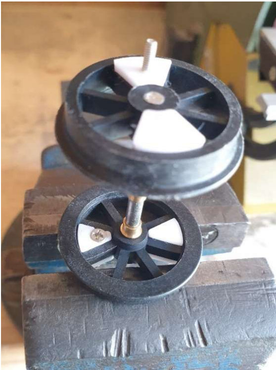
Image is of a loco wheelset (note the longer crankpins on one wheelset, not relevant to the “Nō 9” chassis)
