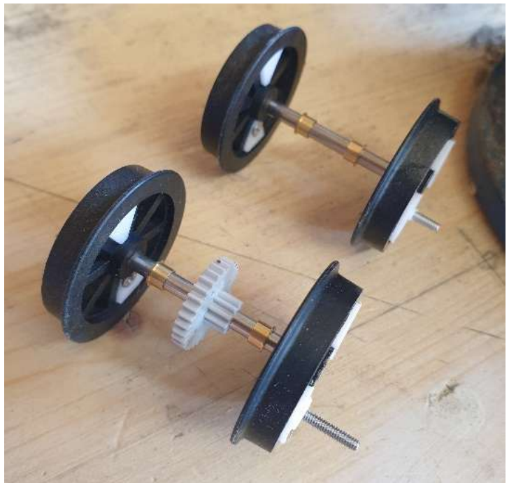
Image is of a loco wheelset (note the longer crankpins on one wheelset, not relevant to the “Nō 9” chassis)
