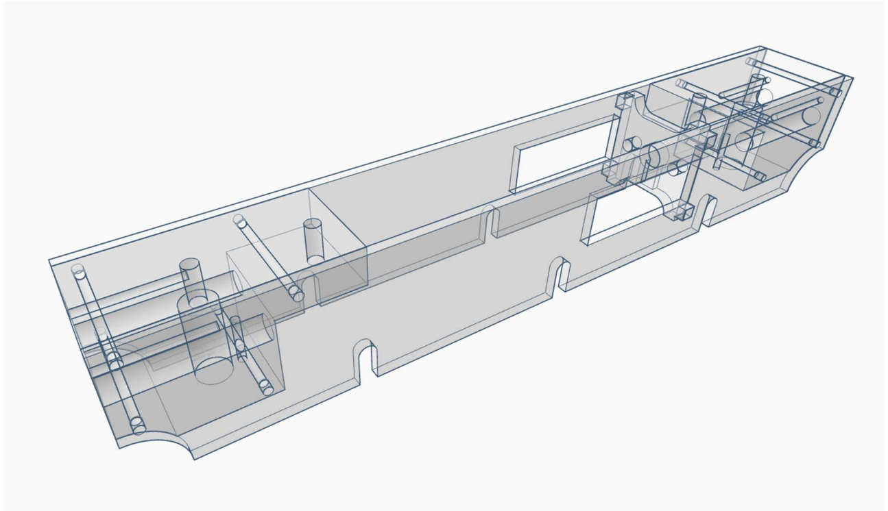
Image is of the 32mm gauge version, the 45mm version just has wider stretchers, motor mount plate & axles.
